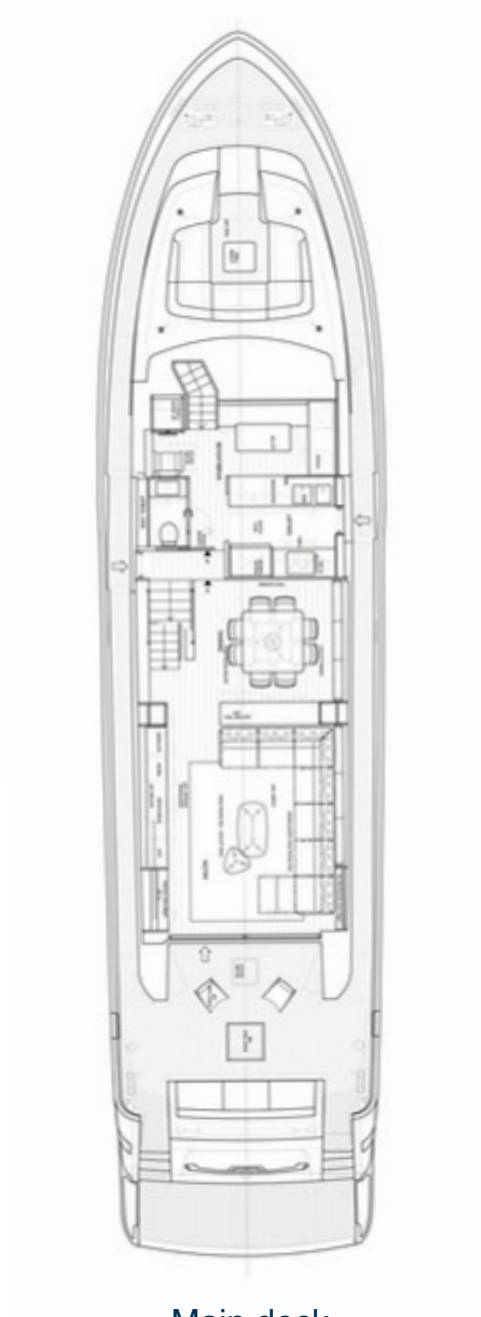
Main deck
